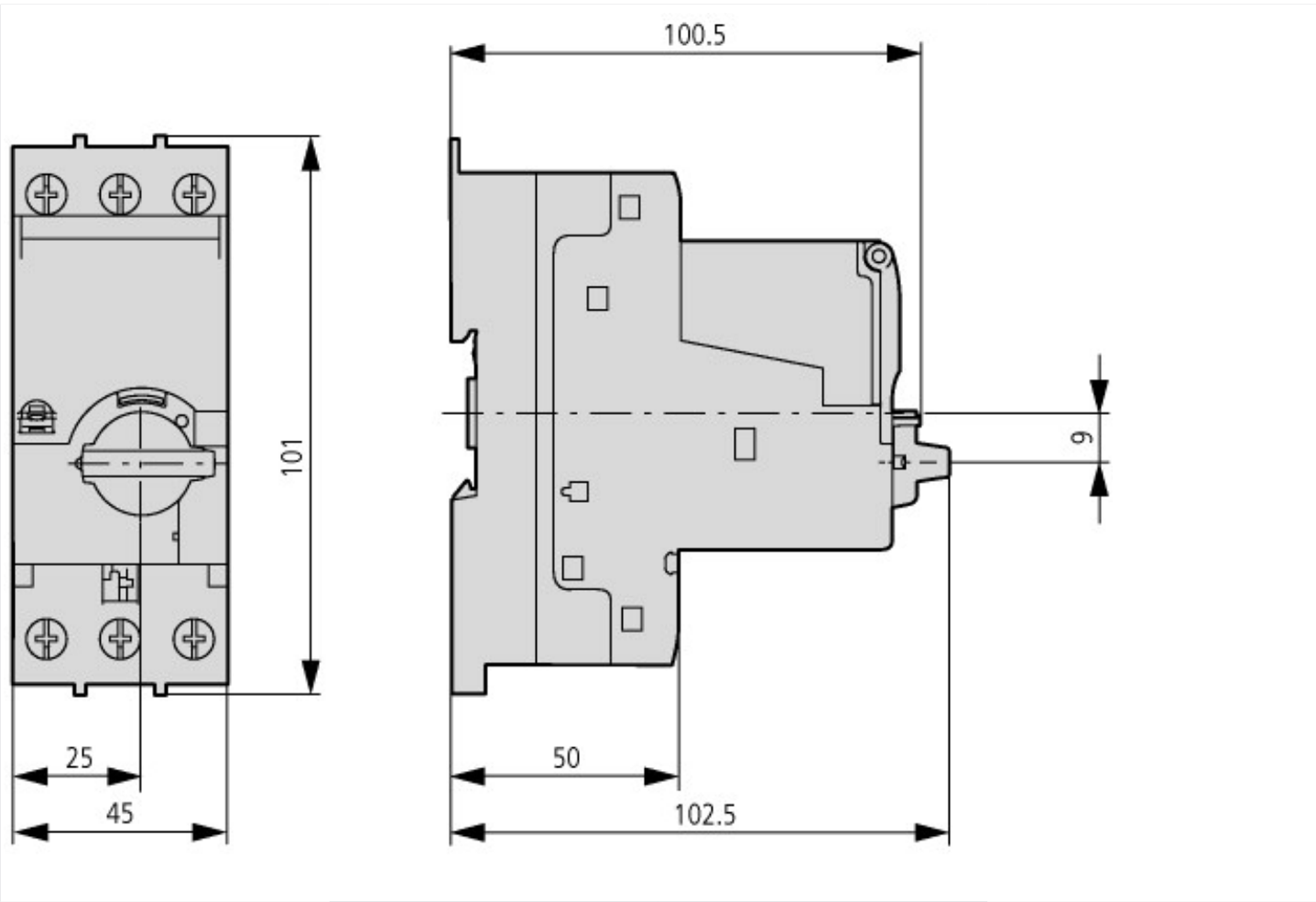
Basic device with trip block
