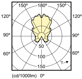
DT 6-40W B22 2200-2700K B38 CL
