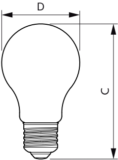
Bulb A60 4.5-40W470lm 2000-2700K D Clear
