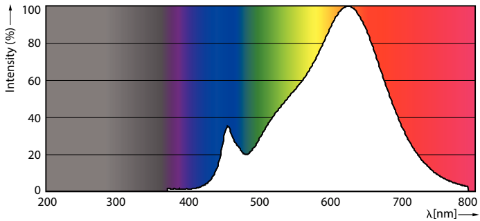
MASTER LEDbulb 40W E27 922-927 FR A60
