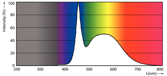
LEDbulb 150W E27 865 FR A80
