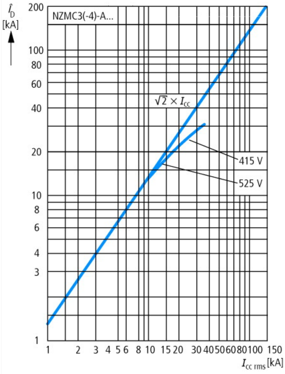
Let-through current
