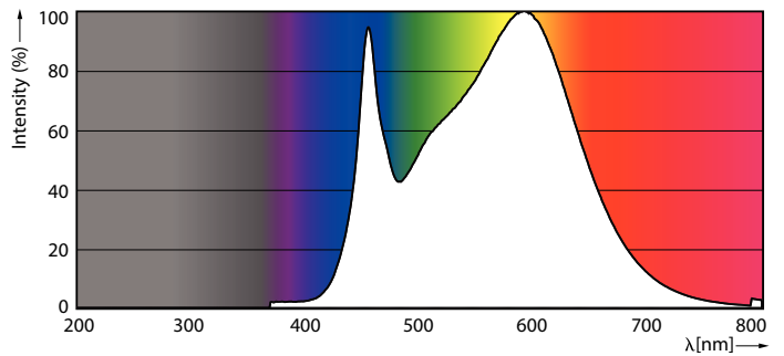
MASTER LEDspotMV 80W GU10 840 36D
