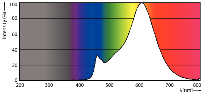
CorePro LEDspotMV 4-42W E27 827 R63
