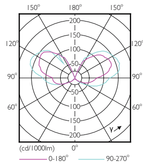
CorePro LEDspotMV 4-42W E27 827 R63
