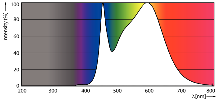
CorePro LEDspotMV 25W GU10 840 36D
