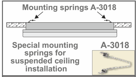
Suspended ceiling installation
